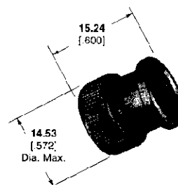
Part No. 413453-1
