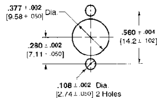
Nickel Plated Part No. 448435-1 Stainless Steel Part No. 448435-2
