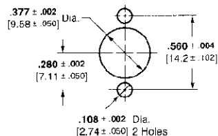
Nickel Plated Part No. 448091-1 Stainless Steel Part No. 448091-2
