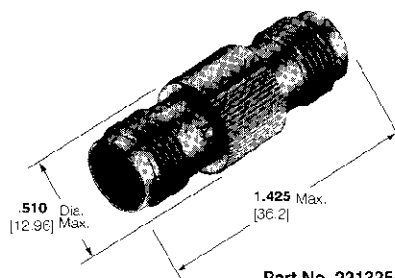
Part No. 221325-1
