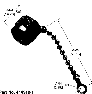
Part No. 414910-1
