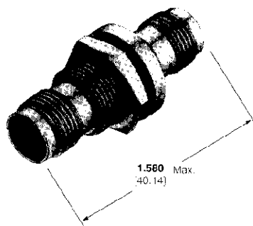
Part No. 221500-1
