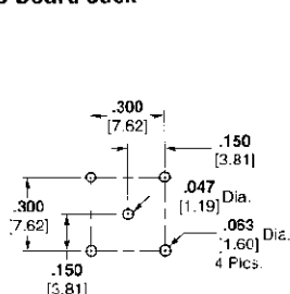
Recommended PC Board Layout "B"
