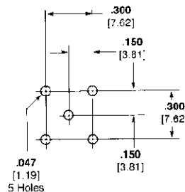
Recommended PC Board Layout "A"
