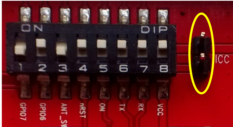
Figure 10: ICC jumper
