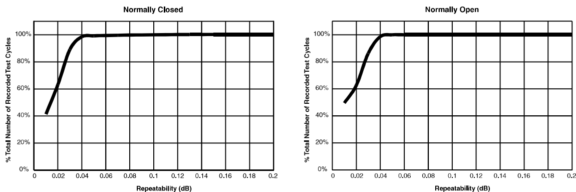
REPEATABILITY CHARACTERISTICS GRF303 RELAYS
