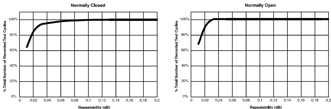
REPEATABILITY CHARACTERISTICS GRF300 RELAYS
