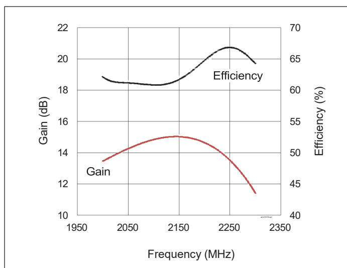
Figure 2. Single-carrier WCDMA Broadband
