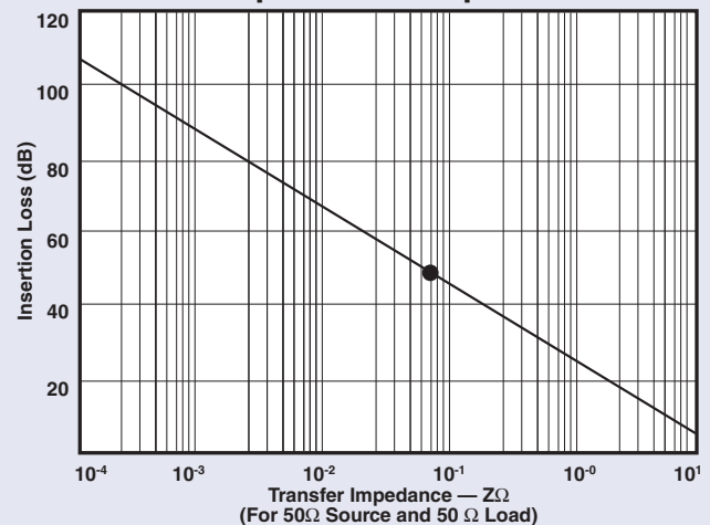
Transfer Impedance Graph
