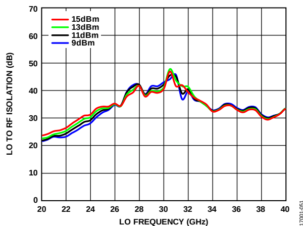
Figure 51. LO to RF Isolation vs. LO Frequency at Various LO Power Levels, T_A = 25^\circ\text{C}
