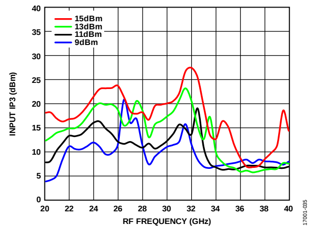
Figure 35. Input IP3 vs. RF Frequency at Various LO Power Levels, T_A = 25^\circ\text{C}
