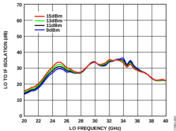
Figure 52. LO to IF Isolation vs. LO Frequency at Various LO Power Levels, T_A = 25^\circ\text{C}
