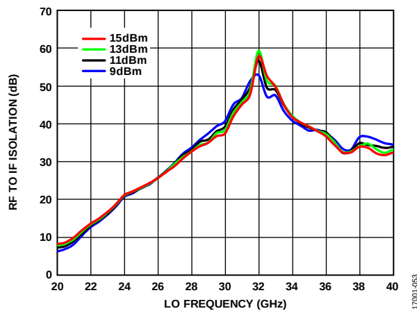
Figure 53. RF to IF Isolation vs. RF Frequency at Various LO Power Levels, T_A = 25^\circ\text{C}
