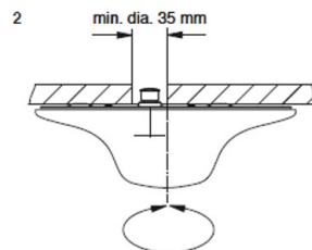
Rotate radome until it locks in place.
