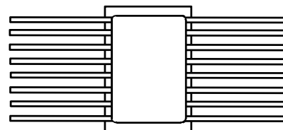
16-PIN Ceramic Flat Pack
