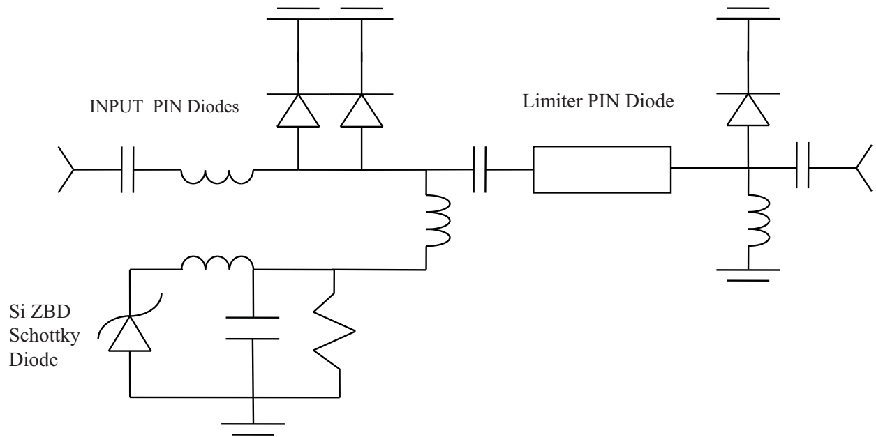
LM202802-Q-B-301 Limiter Schematic
