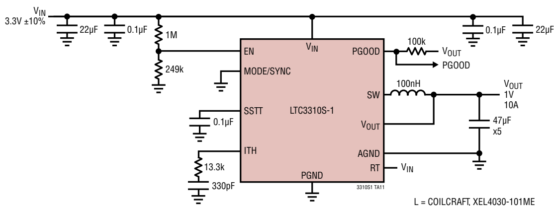
LTC3310S-1, 2MHz, 1.0V, Forced Continuous 1.5A DC to 7.5A Step Load 6A/ \mu s Transient, <3% Total Variation
