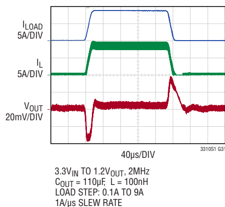
Load Transient Response Pulse-Skipping Mode
