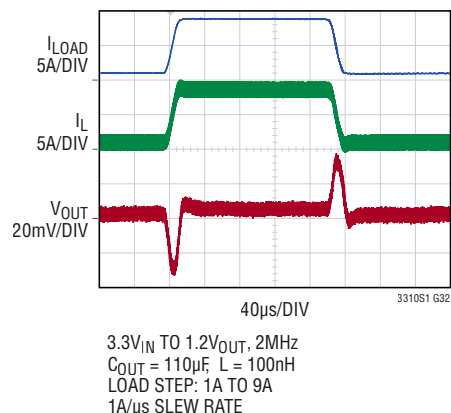
Load Transient Response Forced Continuous Mode
