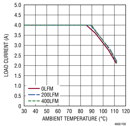
Figure 8. 3.3V to 1.2V Derating Curve, No Heat Sinking
