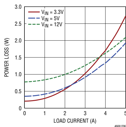
Figure 6. 1.8V Output Power Loss
