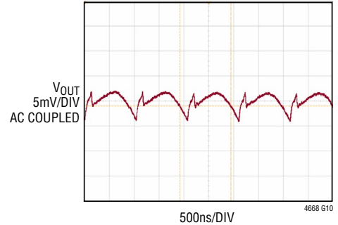
Output Ripple
