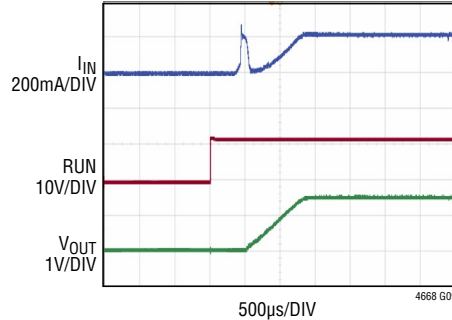
Start-Up with 1.5A Load
