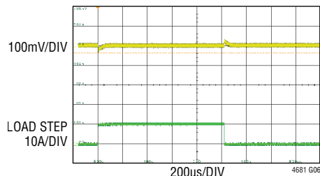
Single Channel Load Transient Response (10A) to (20A) Load Step, 10\text{A}/\mu\text{s} 12\text{V}_{\text{IN}} , \text{V}_{\text{OUT}} = 1.2\text{V} , f_{\text{SW}} = 350\text{kHz}
