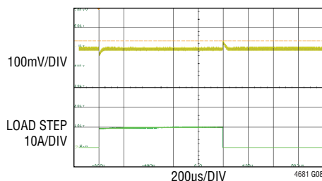
Single Channel Load Transient Response (10A) to (20A) Load Step, 10\text{A}/\mu\text{s} 12\text{V}_{\text{IN}} , \text{V}_{\text{OUT}} = 2.5\text{V} , f_{\text{SW}} = 500\text{kHz}
