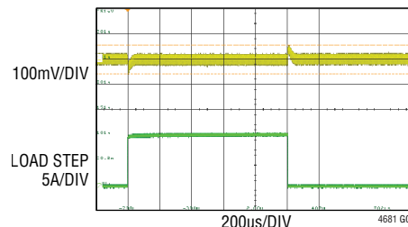
Single Channel Load Transient Response (10A) to (20A) Load Step, 10\text{A}/\mu\text{s} 12\text{V}_{\text{IN}} , \text{V}_{\text{OUT}} = 1.5\text{V} , f_{\text{SW}} = 350\text{kHz}
