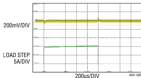
Single Channel Load Transient Response (10A) to (20A) Load Step, 10\text{A}/\mu\text{s} 12\text{V}_{\text{IN}} , \text{V}_{\text{OUT}} = 3.3\text{V} , f_{\text{SW}} = 500\text{kHz}
