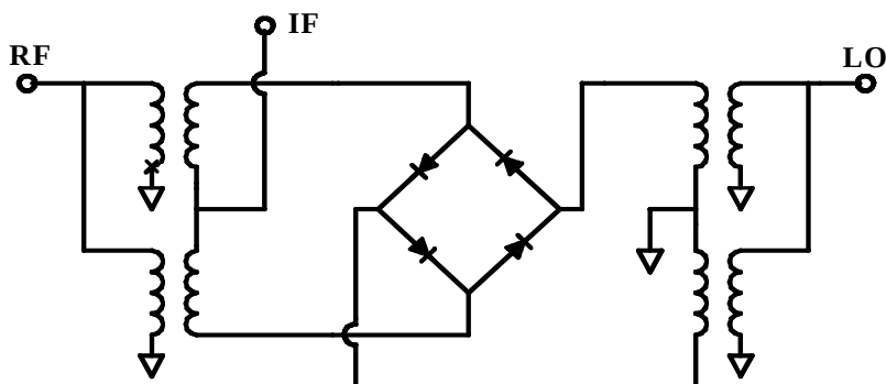
Mixer Schematic
