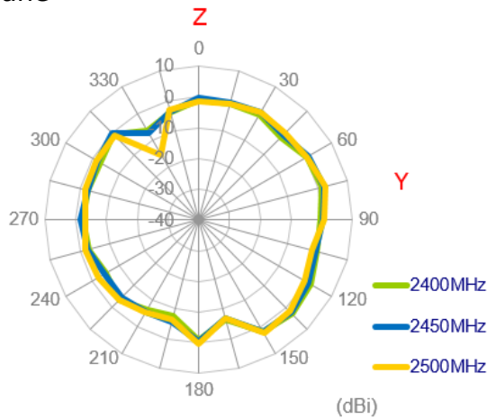
YZ Plane
