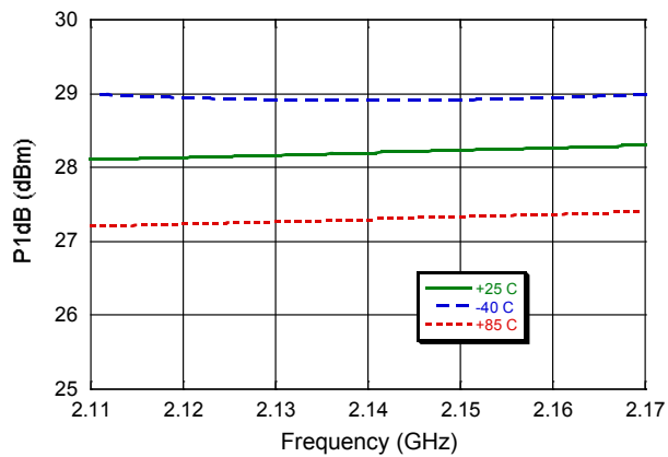
Output P1dB, V_{ctrl} = 0V
