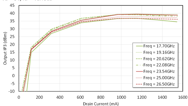
Output IP3 (dBm) vs. Drain Current (mA), V_D = 5\text{ V} , I_D = \text{Various}
