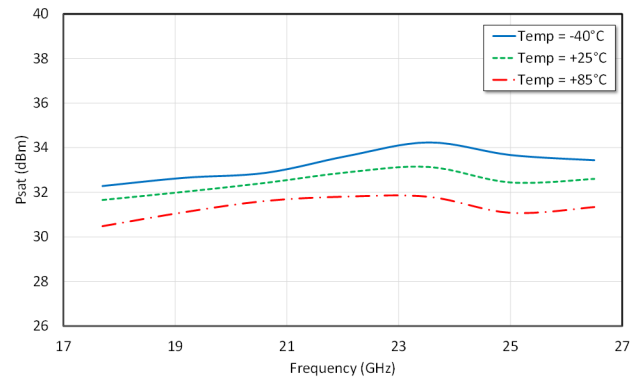
Psat(dBm) vs. Frequency (GHz), V_D = 5\text{ V} , I_D = 1.3\text{ A}
