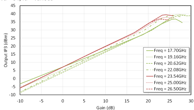
Output IP3 (dBm) vs. Gain (dB), V_D = 5\text{ V} , I_D = \text{Various}
