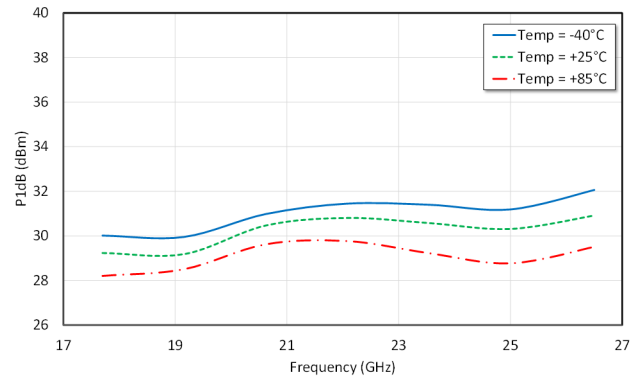
P1dB(dBm) vs. Frequency (GHz), V_D = 5\text{ V} , I_D = 1.3\text{ A}
