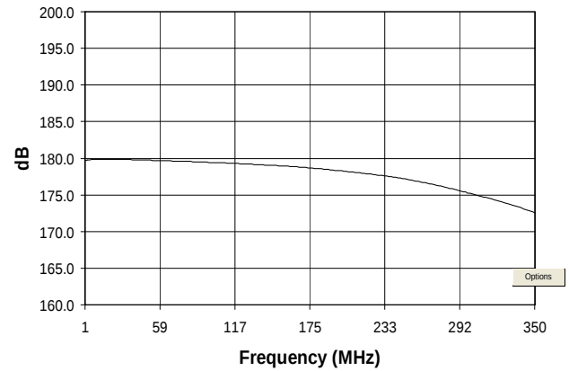
Phase Unbalance
