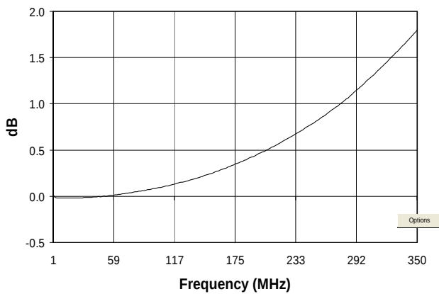
Amplitude Unbalance
