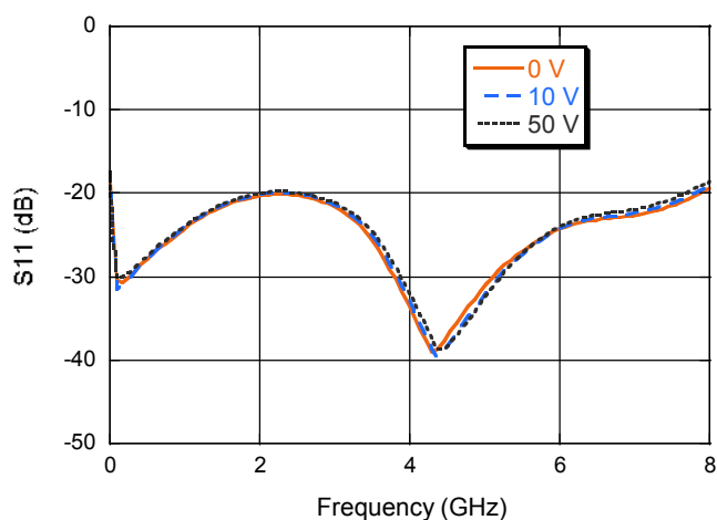
Return Loss
