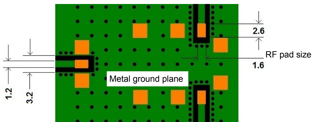
Layout (As viewed from the top side)
