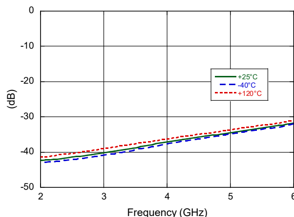
ANT to RX Isolation 10
