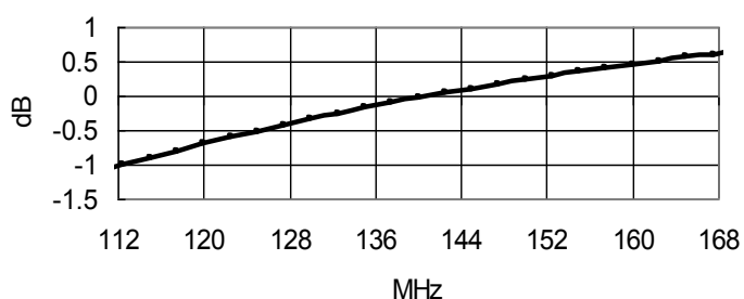
Amplitude Unbalance
