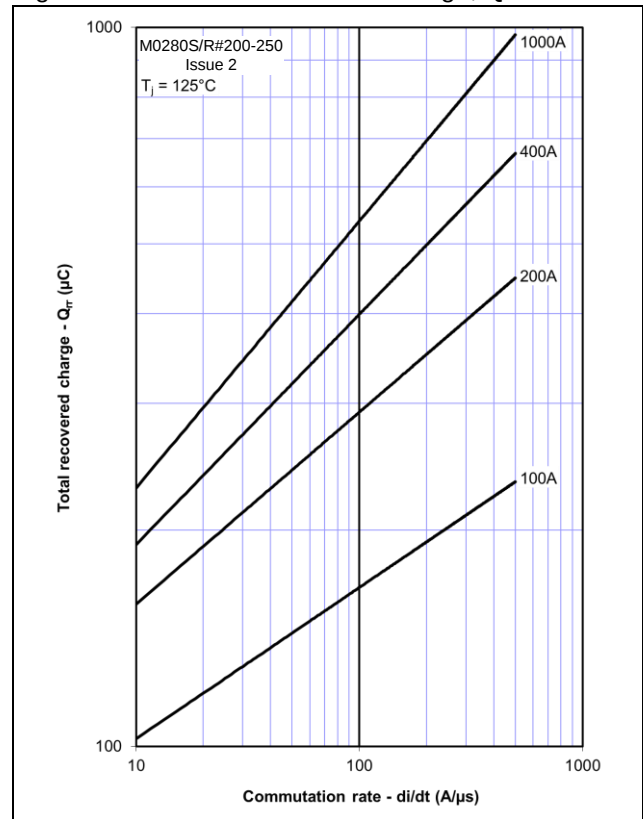
Figure 2 – Maximum recovered charge, Q_{rr}
