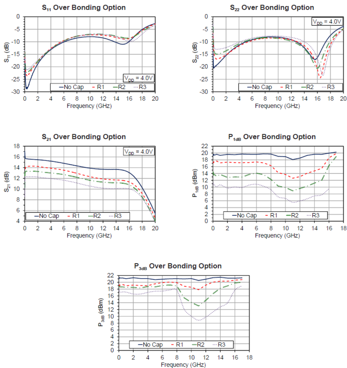
Figure 6 Bonding Option
