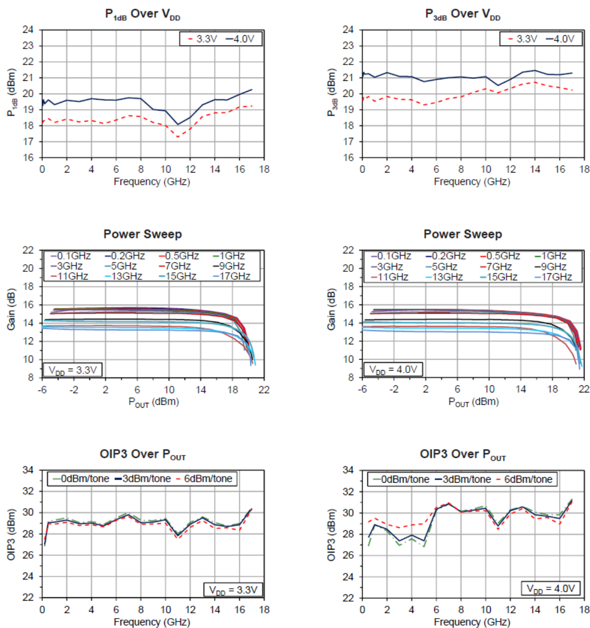
Figure 4 P_{1dB}/P_{3dB} , OIP3, and Power Sweep
