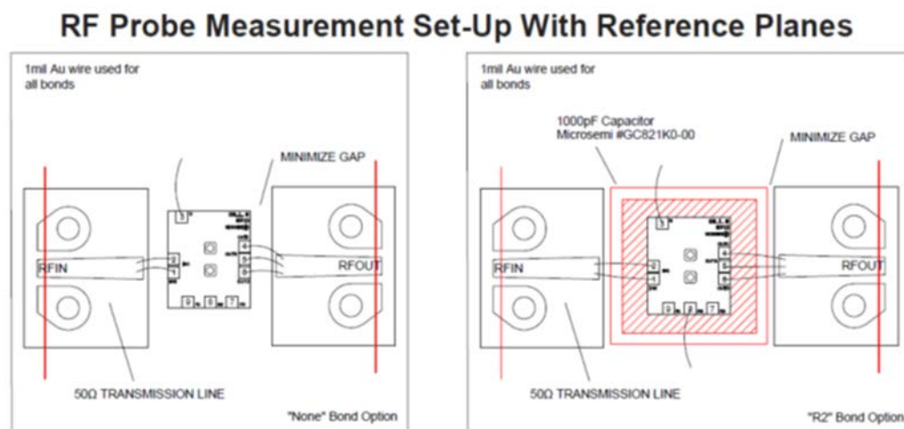
Figure 1 RF Probe Measurement
