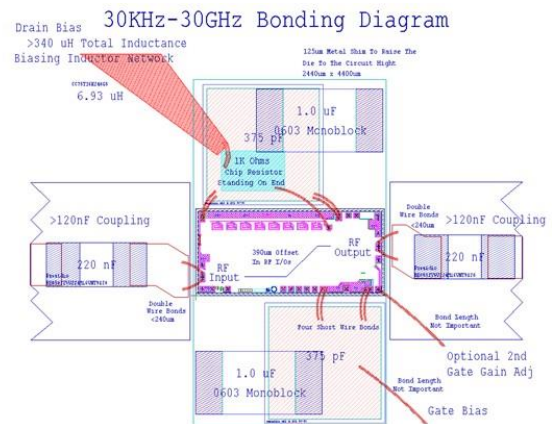
30KHz - 30GHz bonding diagram
