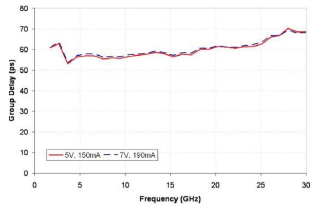
Group Delay
