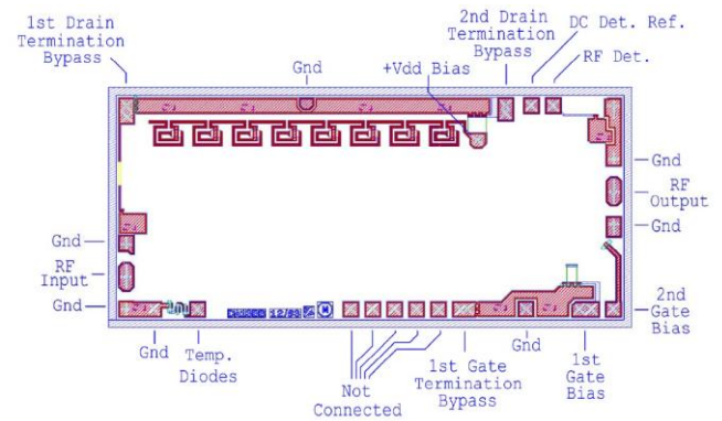
30KHz - 30GHz bonding diagram
