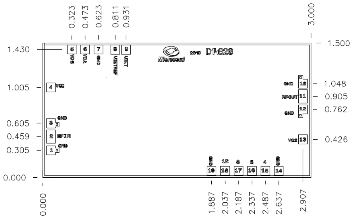
Figure 20 Outline Package
