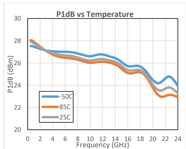
Figure 11 P1dB vs Temperature ( V_{DD} = 10\text{ V} , I_{DD} = 235\text{mA} )
