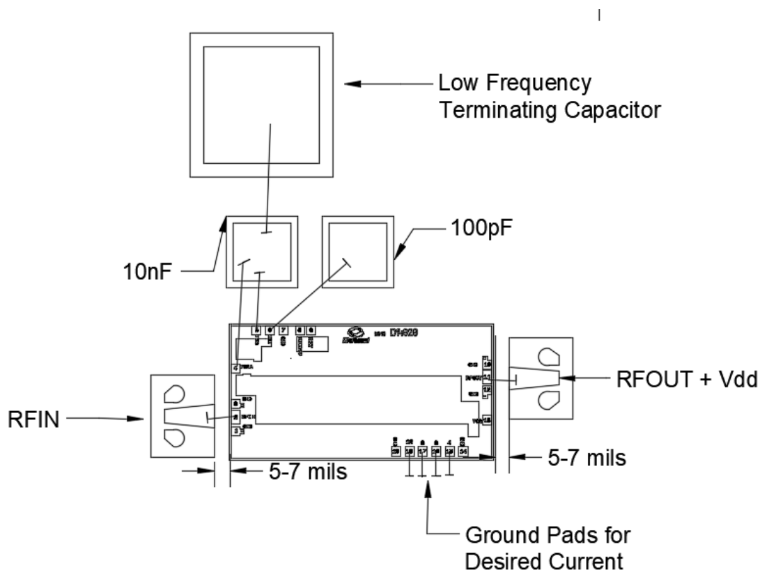
Figure 22 Assembly Diagram
