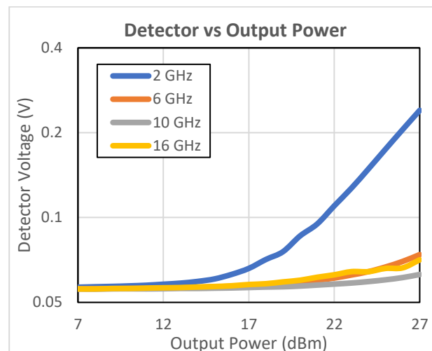
Figure 19 Detector Voltage vs Output Power ( V_{DD} = 10\text{ V} , I_{DD} = 235\text{mA} , T = 25\text{ }^{\circ}\text{C} )
