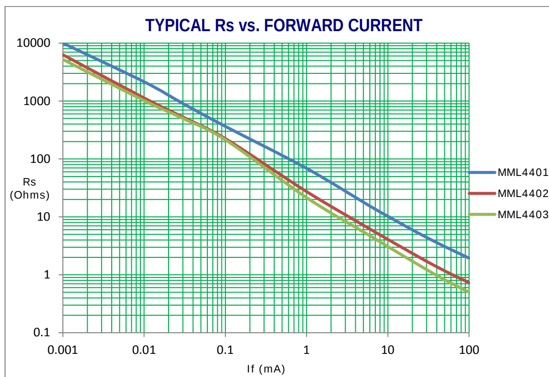
Figure 3 Typical R_s Performance
