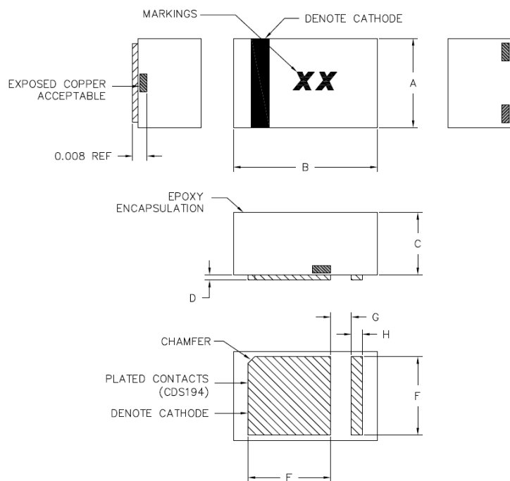
Figure 4 GM2 Package Outline
