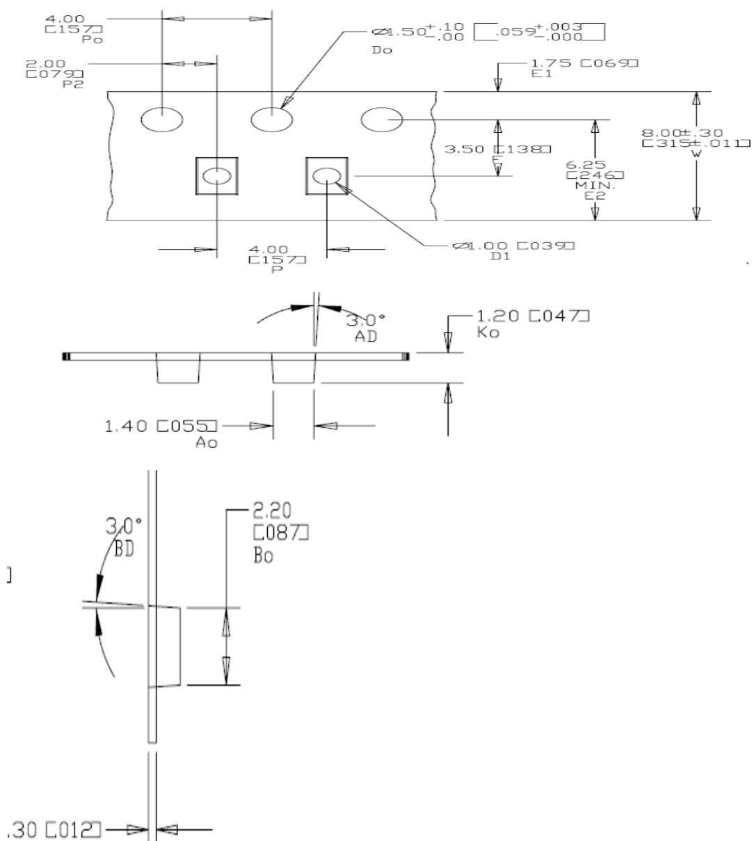
Figure 6 GM2 Tape-and-Reel Format
