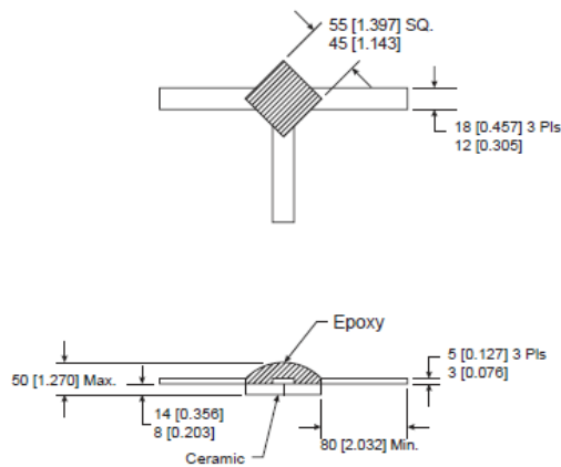
E35 (non-hermetic)
