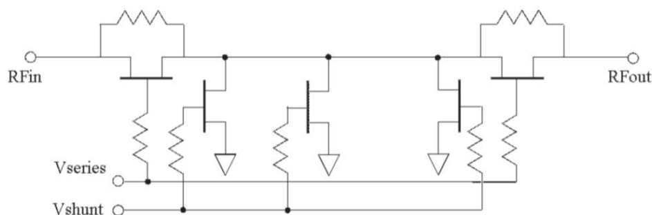
Figure 6: UVD50SC Simplified Schematic Diagram
