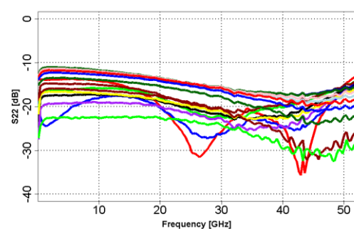
Figure 4: Typical on wafer measured performance
