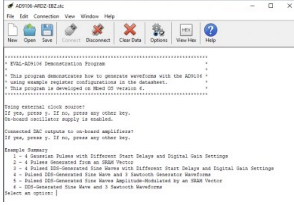
Figure 9a. EVAL-AD9106 Demo Program Menu | Figure 9b. EVAL-AD9102 Demo Program Menu
