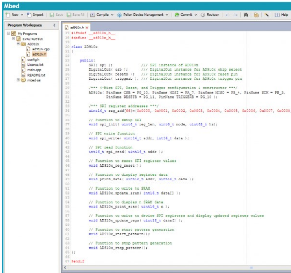
Figure 20. Device-specific I/O pins and functions declarations in ad910x.h
