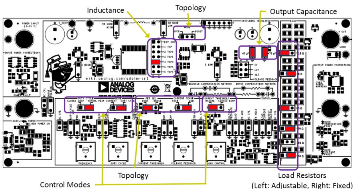
Figure 2. Topology, Mode selection, and Loads
