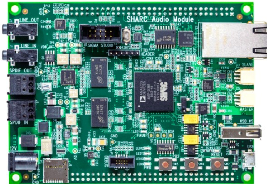
The SHARC Audio Module Main Board
