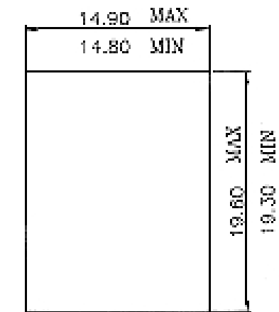
Single Panel-Latch Clearance Panel Thickness 0.062 inch
