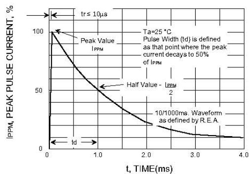
FIG.5 - PULSE WAVEFORM
