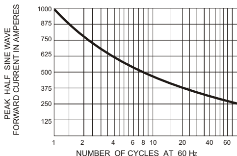
Figure 2 NON-REPETITIVE SURGE CURRENT
