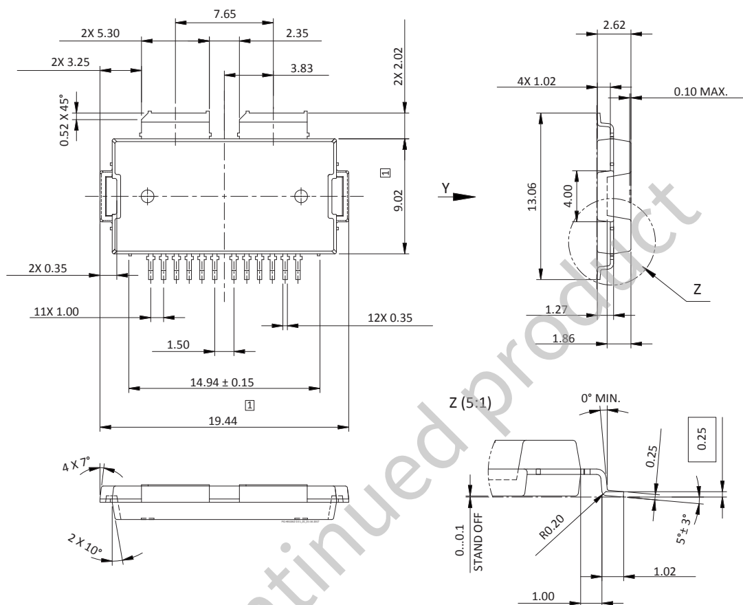
Package PG-HB1DSO-14-1 (formed leads)
