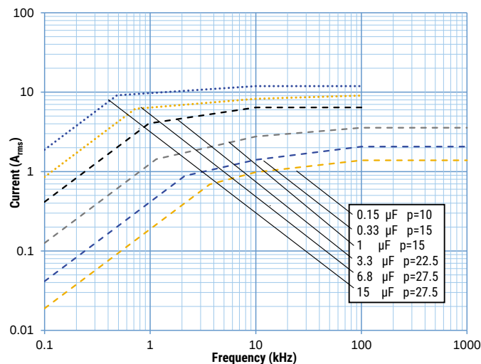
520 VDC/200 VAC
