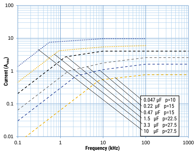
630 VDC/220 VAC
