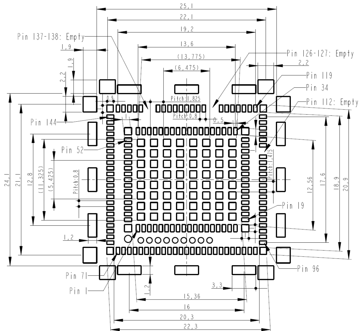
Figure 8. Recommended WP Series Snap-in Socket Footprint – Copper Layout Position
