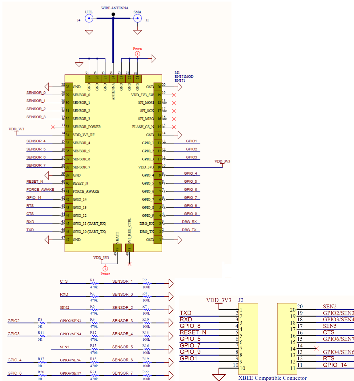
Figure 1. Application Schematic
