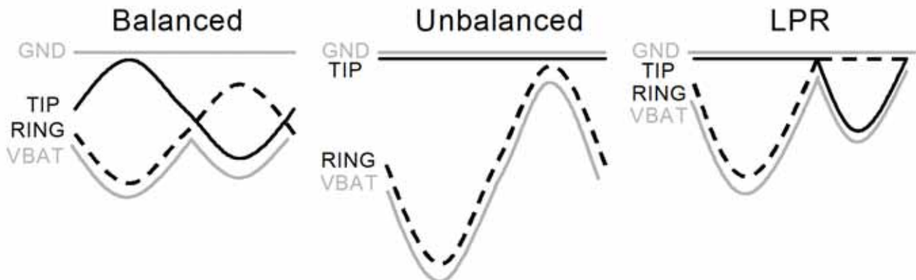
Figure 26. Ringing Modes
