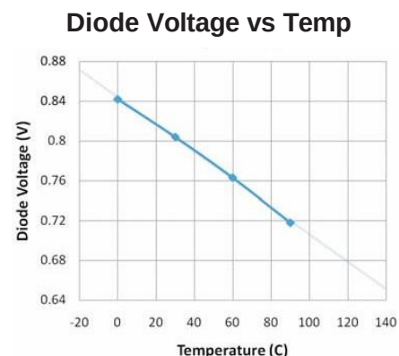
Diode Voltage vs Temp, I_d = 120 \mu A T = (0.84 - V_d) / 0.00133
