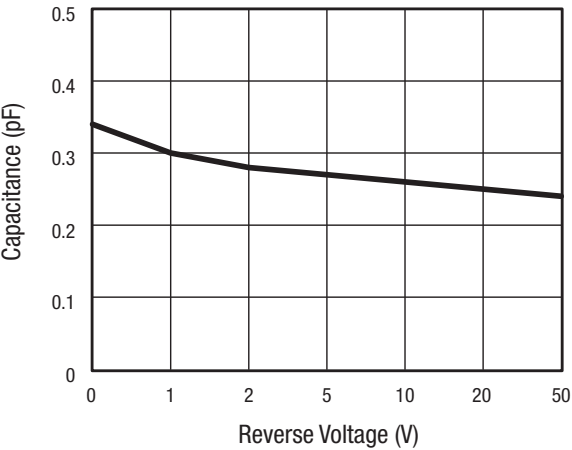
Figure 4. Capacitance vs Reverse Voltage (1 MHz to 1 GHz)
