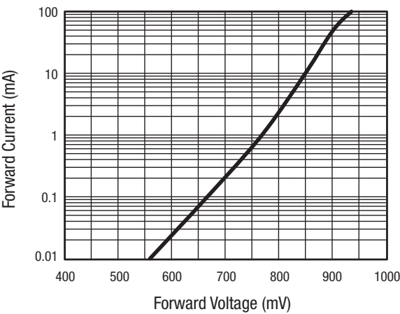
Figure 3. DC Characteristics
