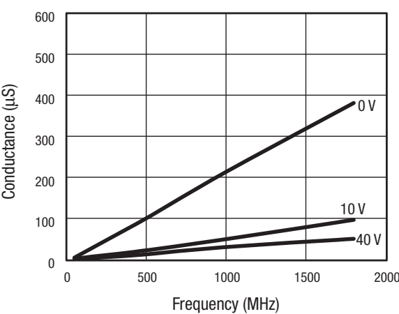
Figure 5. Conductance vs Frequency and Reverse Voltage
