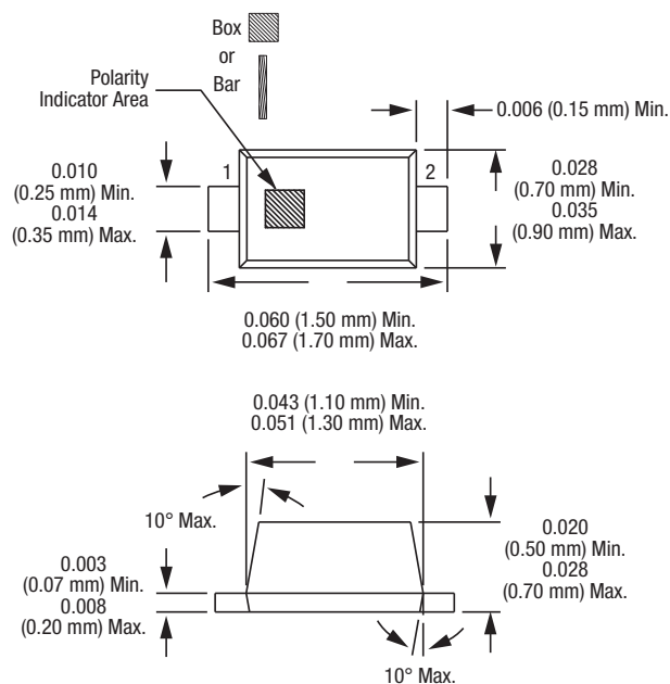
Figure 8. SC-79 Package Dimension Drawing
