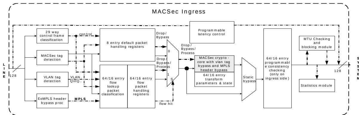
Figure 39 • MACsec Ingress Data Flow
