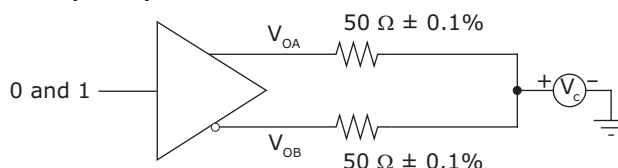
Figure 88 • SGMII DC Driver Output Impedance Test Circuit
