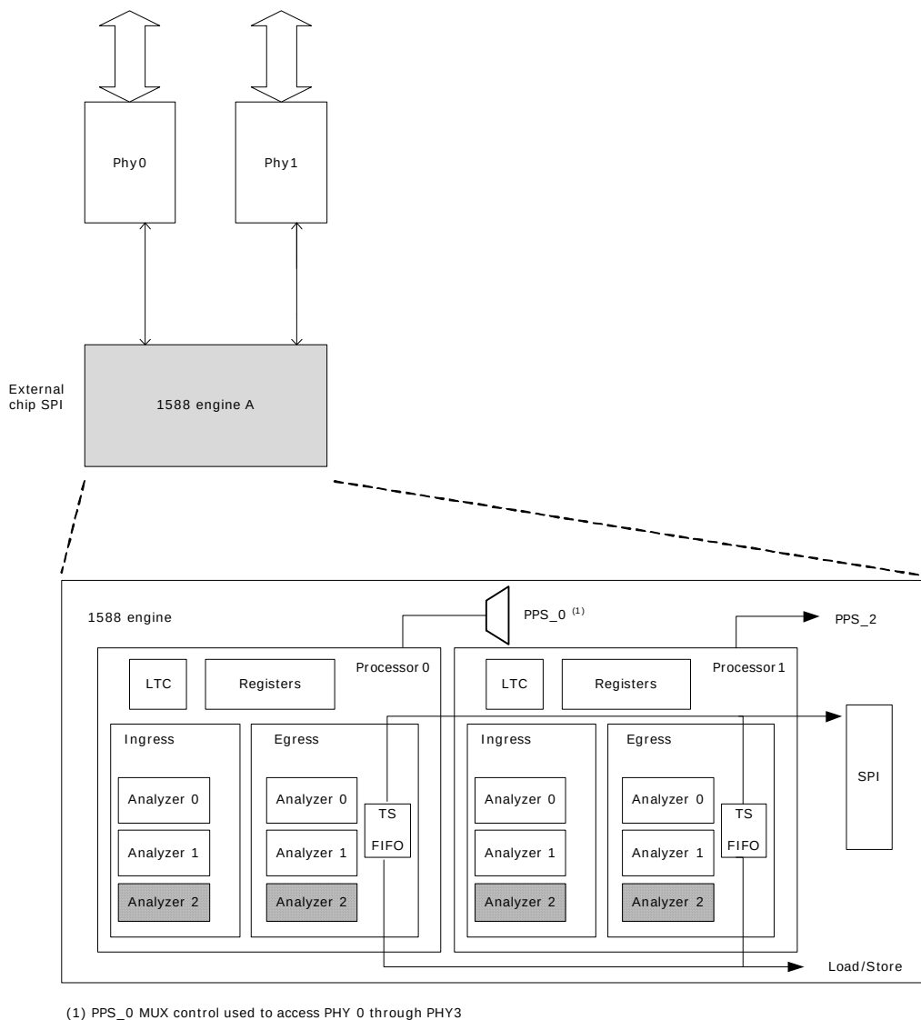
Figure 18 • IEEE 1588 Architecture
