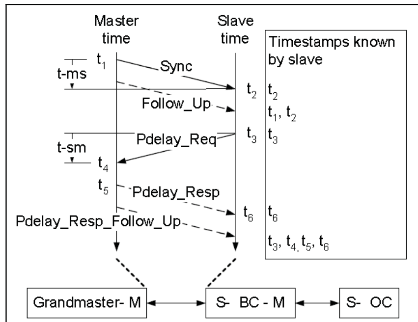
Figure 25 • Delay Measurements
