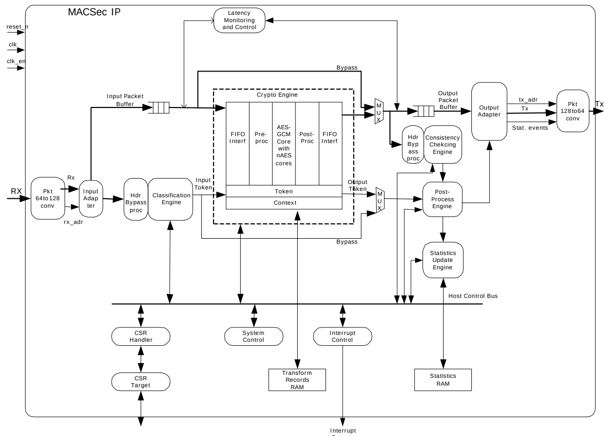
Figure 64 • MACsec Architecture
