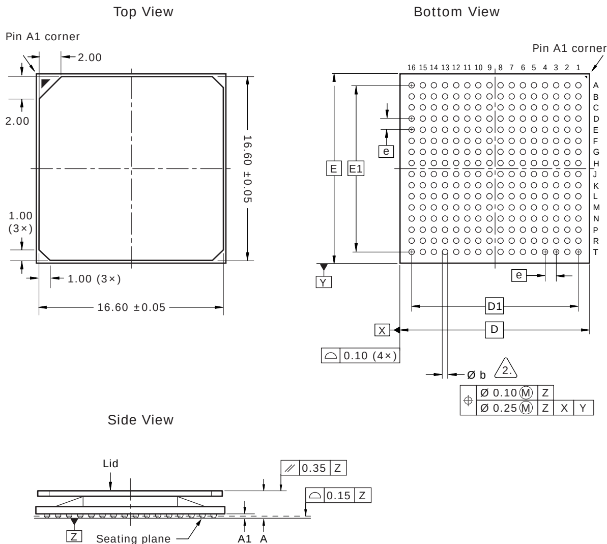
Figure 124 • VSC8254-01 Package
