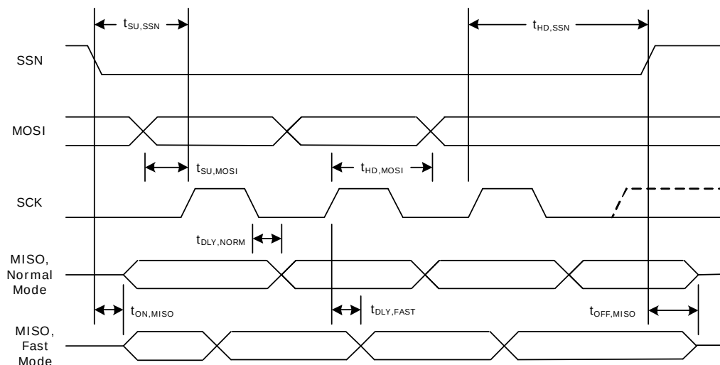
Figure 27 • SPI Interface Timing
