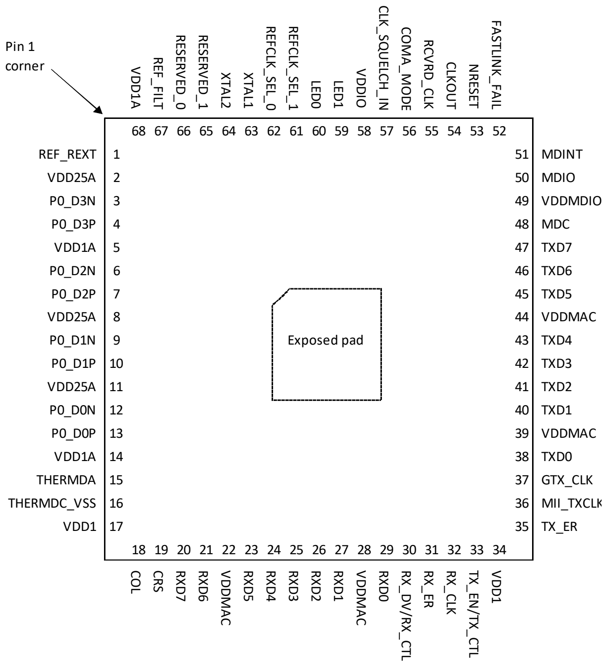
Figure 35 • Pin Diagram
